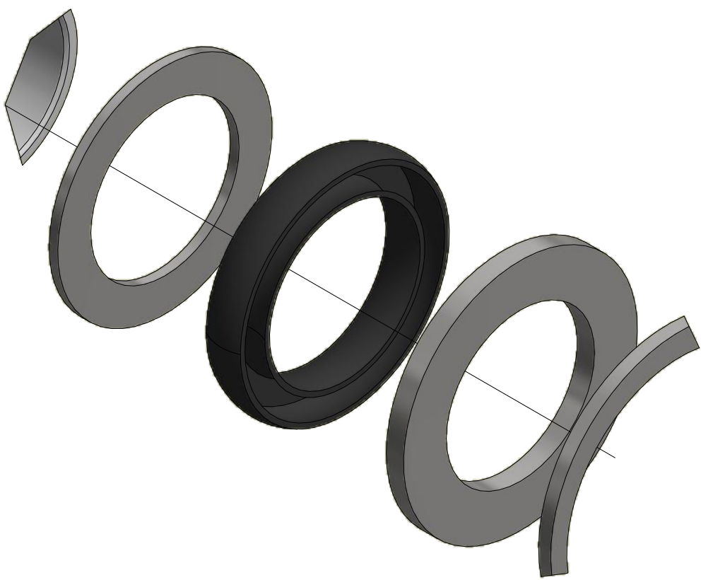
DETAIL B NOTE ORIENTATION OF SEAL & ADDITION OF THRUST BEARING
