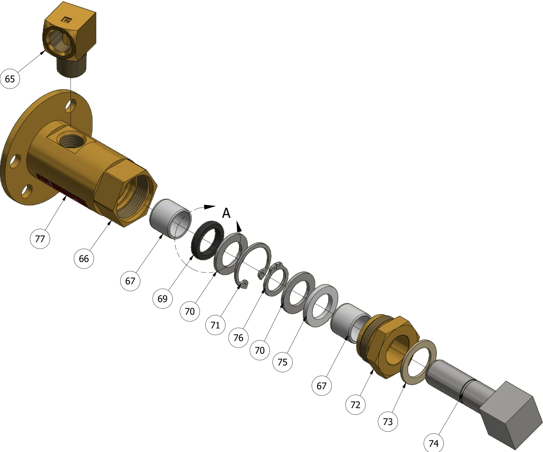
FOR AIR SYSTEMS
