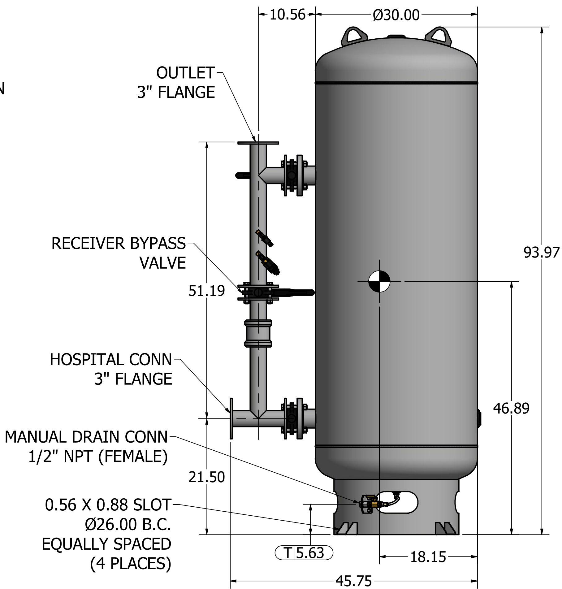
240 GAL VACUUM RECEIVER 3" FLANGED CONNECTIONS (SCALE 1:11)
