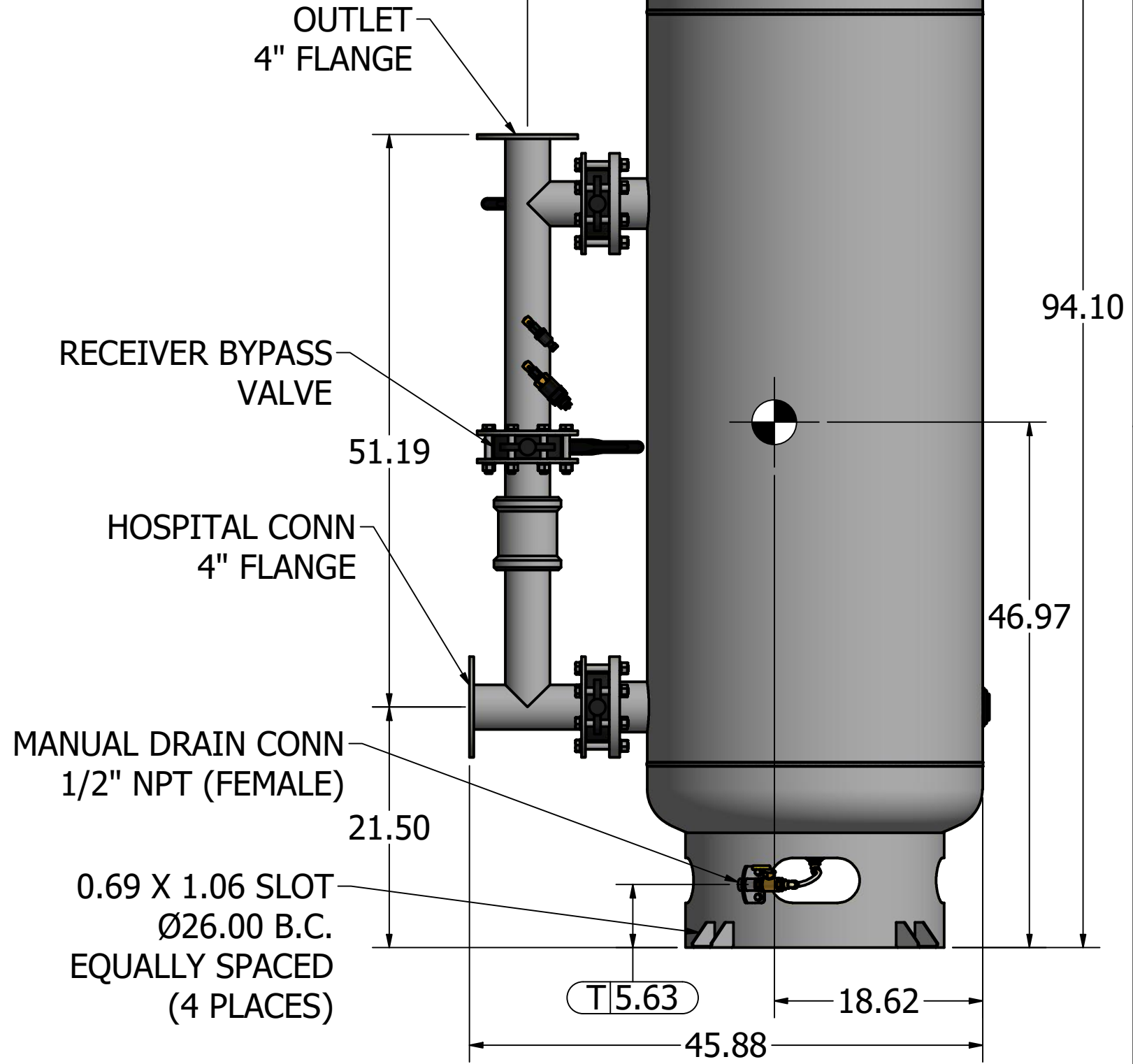
240 GAL VACUUM RECEIVER 4" FLANGED CONNECTIONS (SCALE 1:12)
