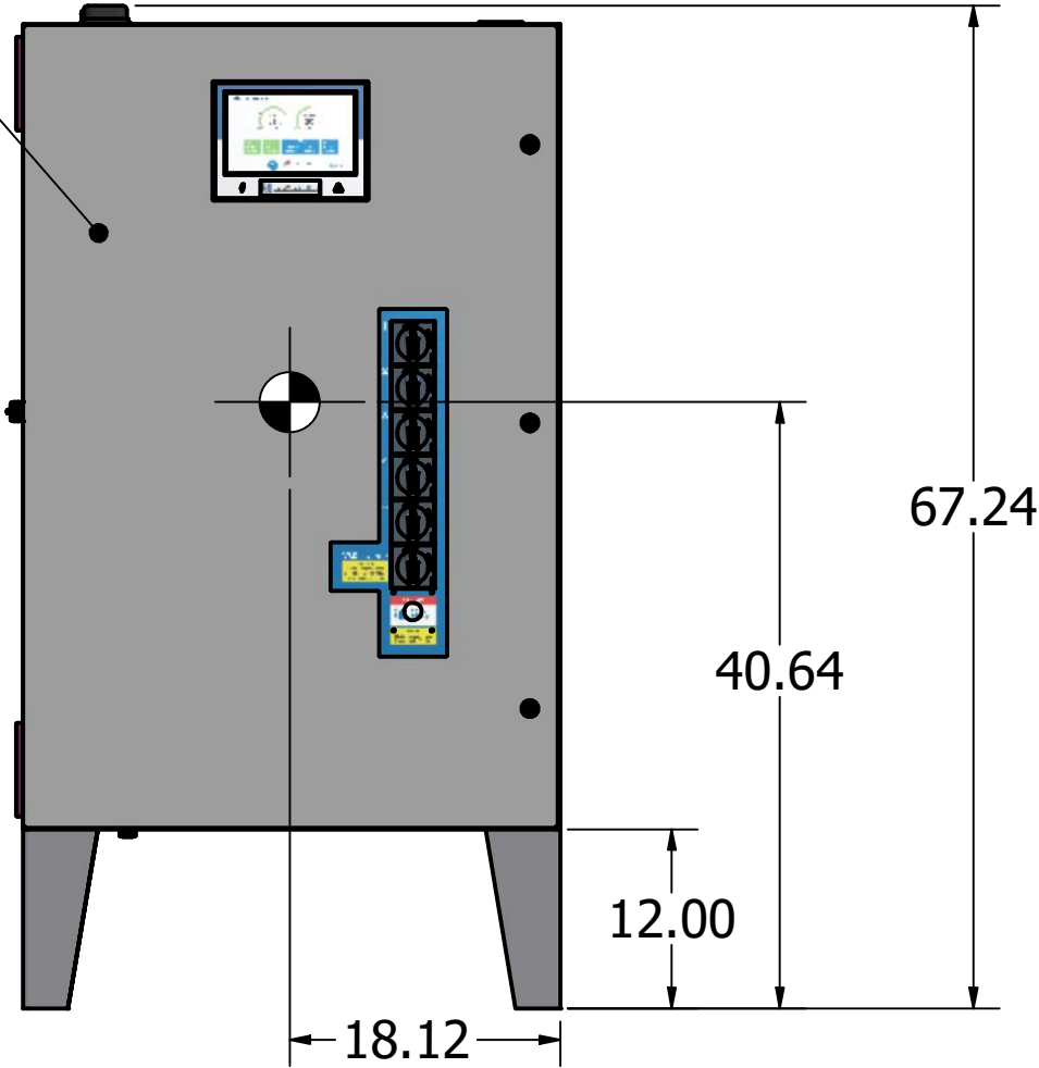
CONTROL CABINET
