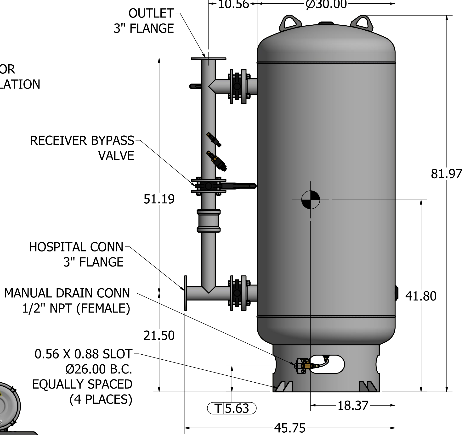
200 GAL VACUUM RECEIVER 3" FLANGED CONNECTIONS (SCALE 1:10)
