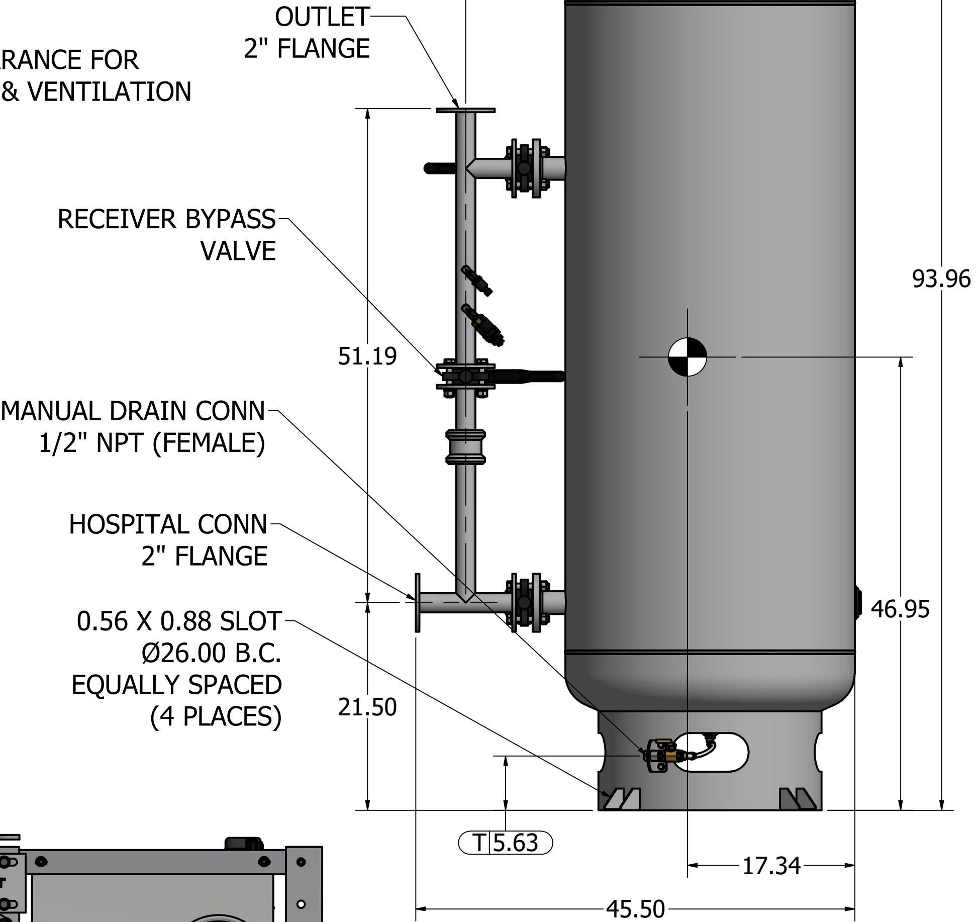
240 GAL VACUUM RECEIVER 2" FLANGED CONNECTIONS (SCALE 1:10)
