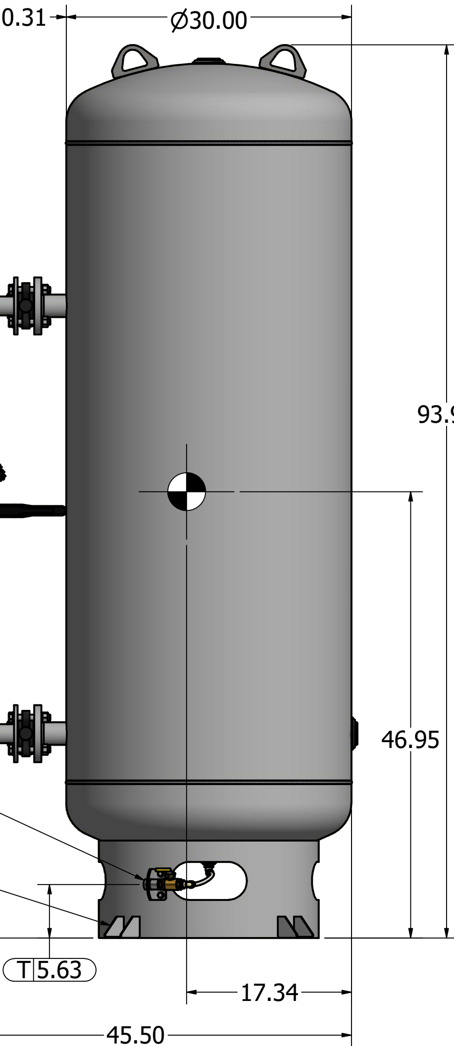
240 GAL VACUUM RECEIVER 2" FLANGED CONNECTIONS (SCALE 1:10)
