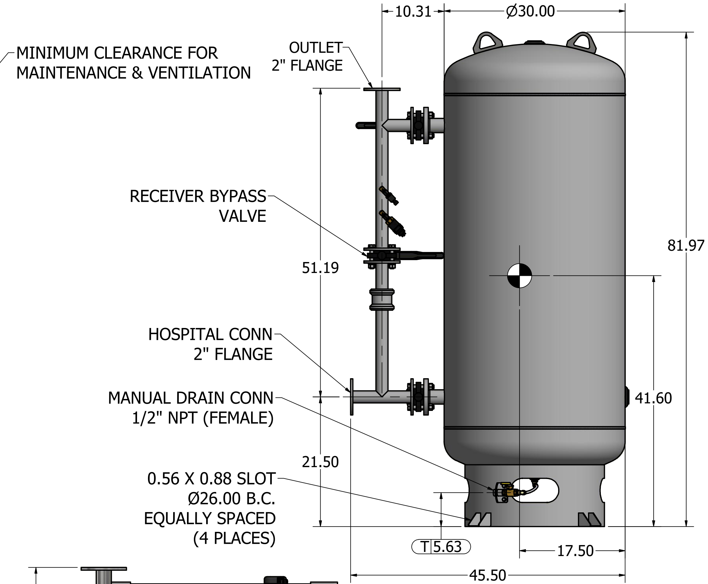
200 GAL VACUUM RECEIVER 2" FLANGED CONNECTIONS (SCALE 1:10)
