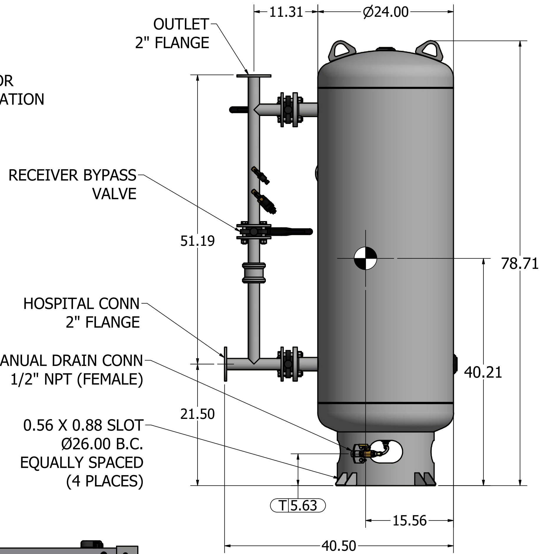
120 GAL VACUUM RECEIVER 2" FLANGED CONNECTIONS (SCALE 1:10)
