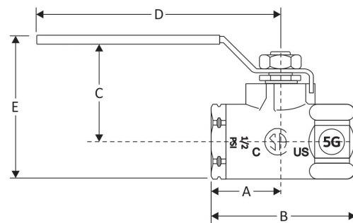
1/8" F.NPT Tapping Port Shown Open But Shipped with Pipe Plug Installed
