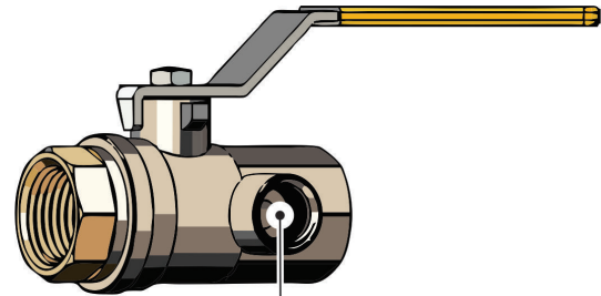
1/8" F.NPT Tapping Port Shown Open But Shipped with Pipe Plug Installed
