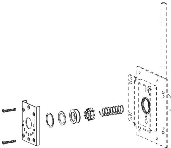
Figure 1: DiamondCare® Pressure Recessed Wall Outlet Conversion Kit - P/N 4107 2011 99
