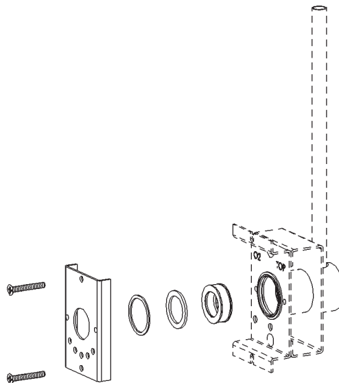
Figure 4: DiamondCare ® Vacuum Console Outlet Conversion Kit - P/N 4107 2012 02
