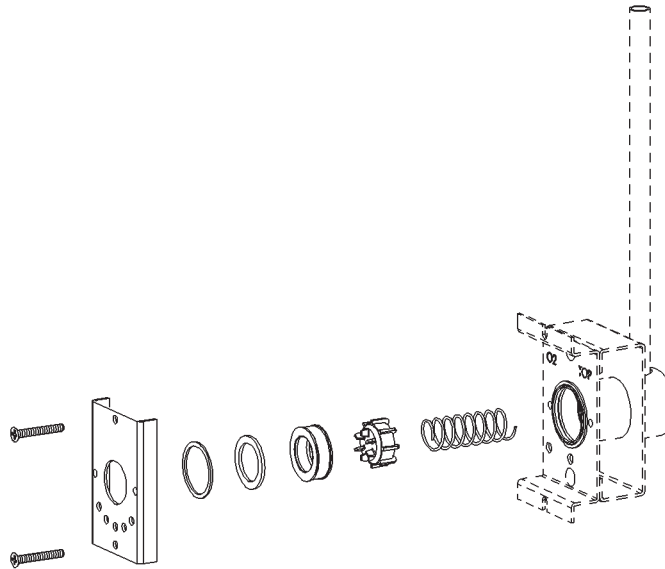
Figure 3: DiamondCare ® Pressure Console Outlet Conversion Kit - P/N 4107 2012 01
