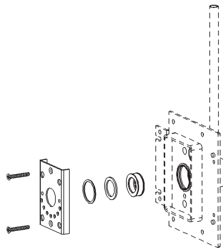
Figure 2: DiamondCare® Vacuum Recessed Wall Outlet Conversion Kit - P/N 4107 2012 00
